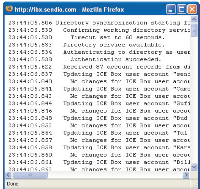
[62] Directory Synchronization
