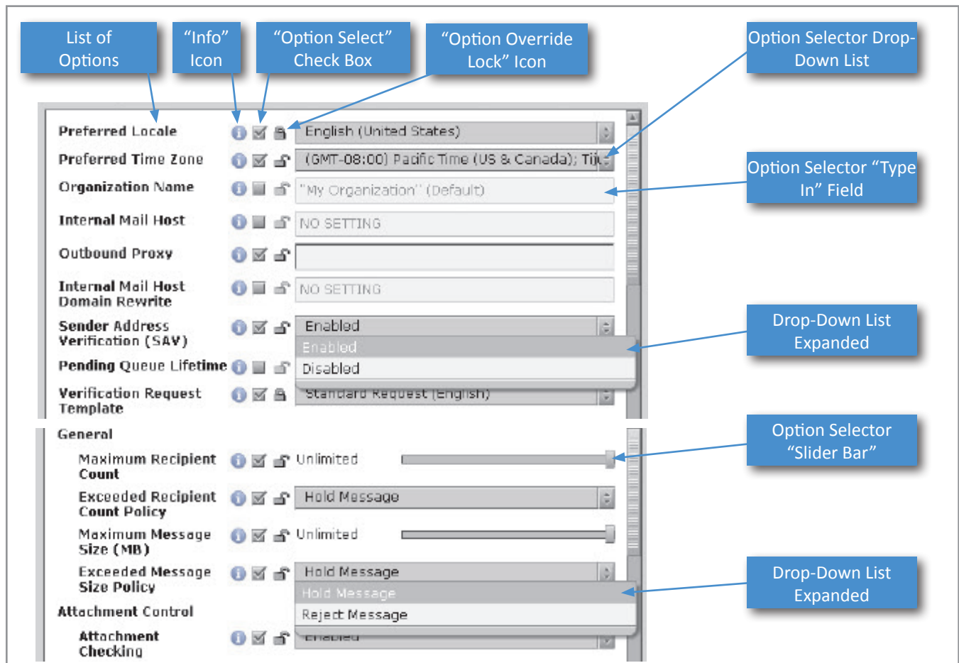
[16] List-Oriented Controls
