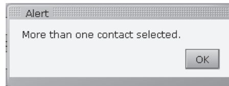
[34] Alert Dialog
