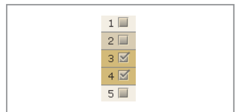
[12] Check boxes
